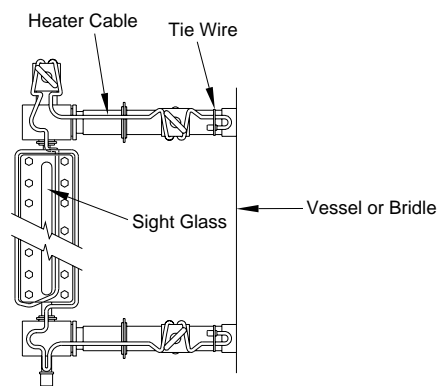
Figure 20 Level Gauge
