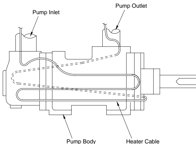
Figure 18 Pump
