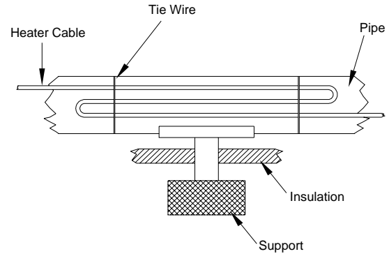
Figure 13 Support
