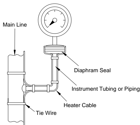
Figure 19 Pressure Indicator
